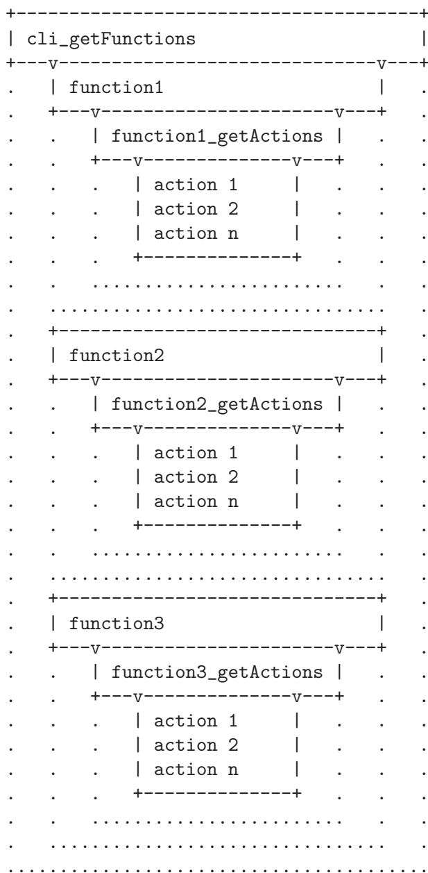
Figure 3.2: The actions initialization environment.
